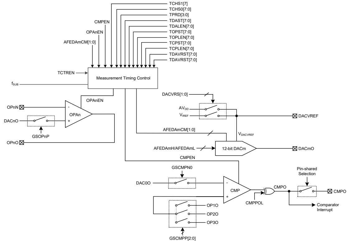
测量电路方框图 (m=0~3, n=1~3)
