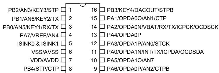
BS45F3340/BS45V3340 16 NSOP-A
