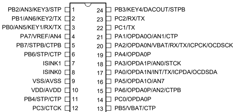
BS45F3340/BS45V3340 24 SSOP-A
