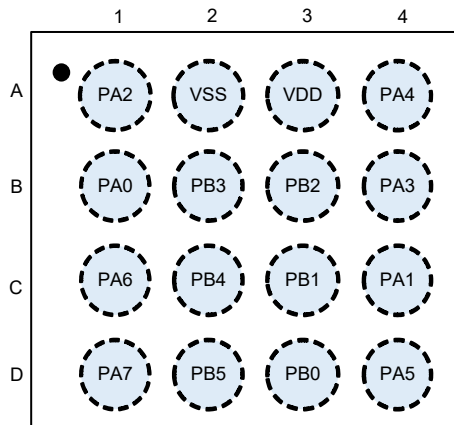
BS84B04C 16 WLCSP-A
