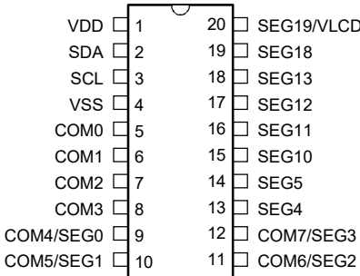
HT16C21A 20 SOP-A/SSOP-A
