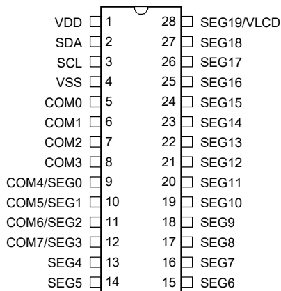
HT16C21A 28 SOP-A/SSOP-A
