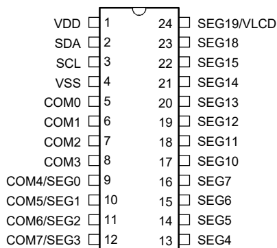
HT16C21A 24 SOP-A/SSOP-A
