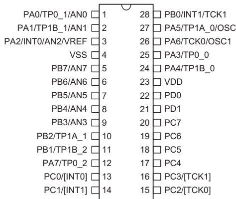
HT66F25D 28 SOP-A LED 8x8 (Source/Sink)
