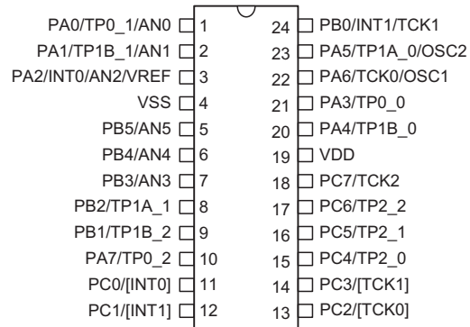
HT66F26D 24 SOP-A LED 8x6 (Source/Sink)
