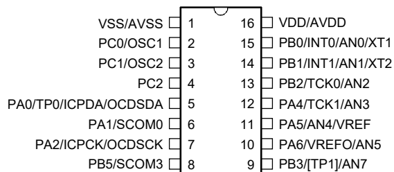
HT66F317/HT66V317 16 NSOP-A
